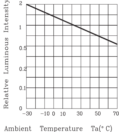
LUMINOUS INTENSITY VS AMBIENT TEMPERATURE
