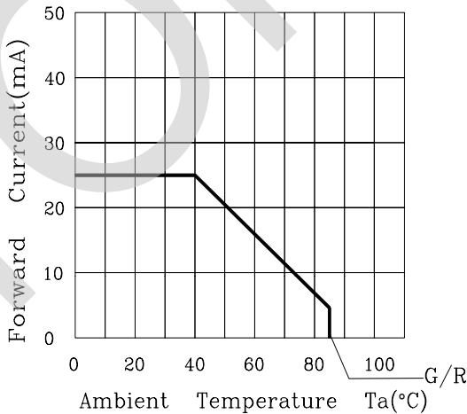
FORWARD CURRENT VS DERATING CURVE
